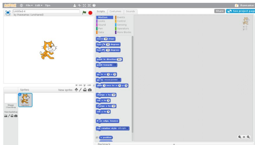
Figure 3. Scratch IDE
